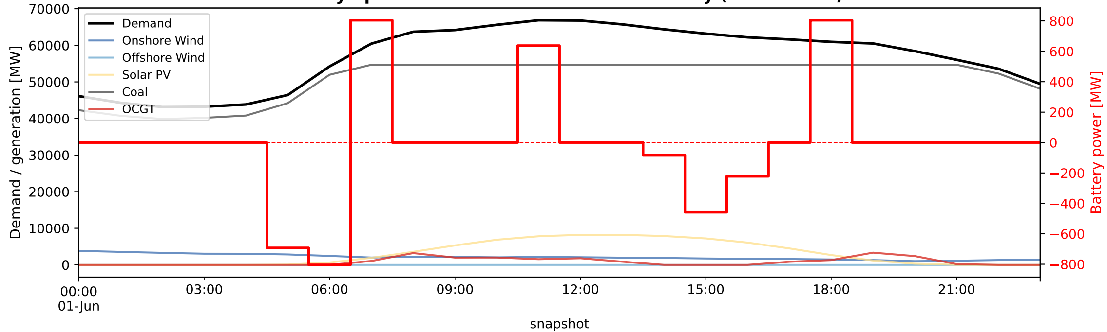
Battery operation on most active summer day (2017-06-01)
